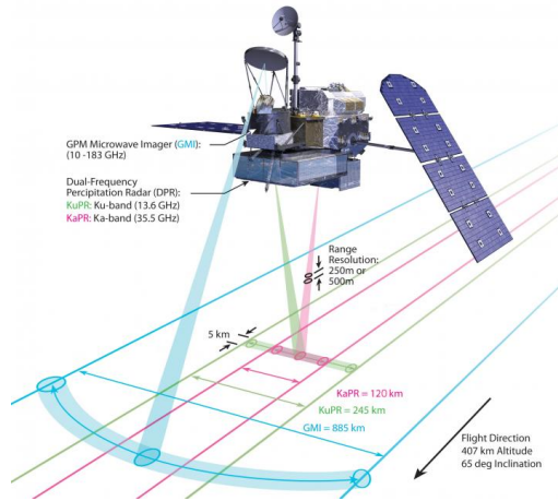
The GPM Core Observatory carries the first space-borne Ku/ (DPR) and a multi-channel (GMI).
